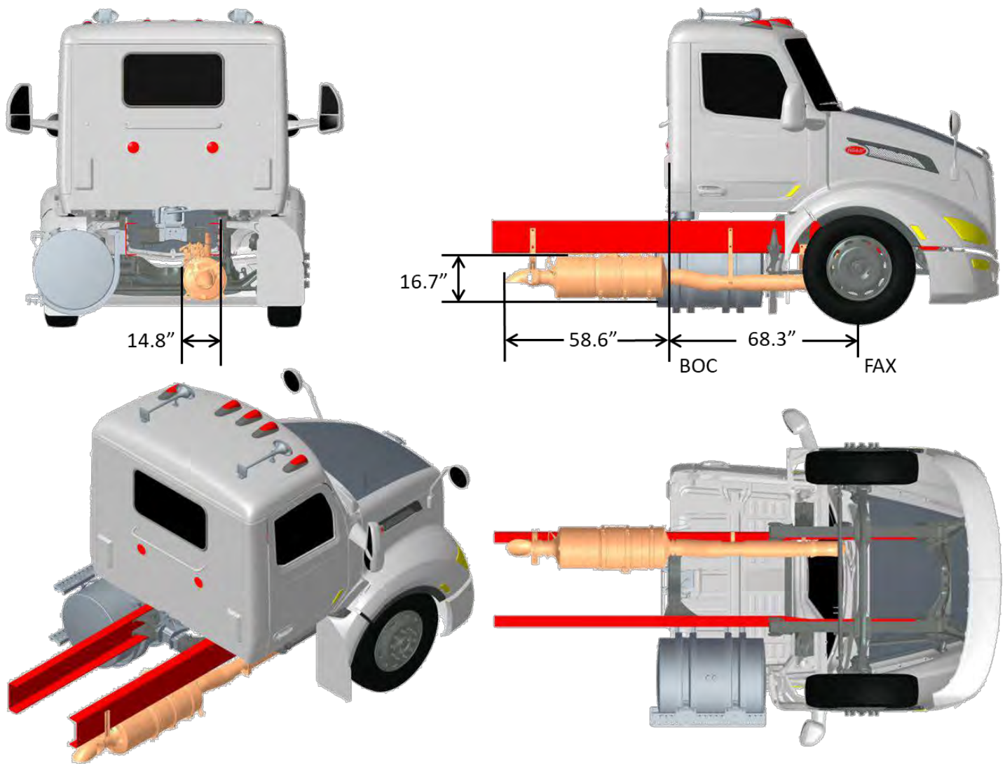
FIGURE 3-99. Exhaust Single RH Horizontal DPF/SCR RH Under Frame
