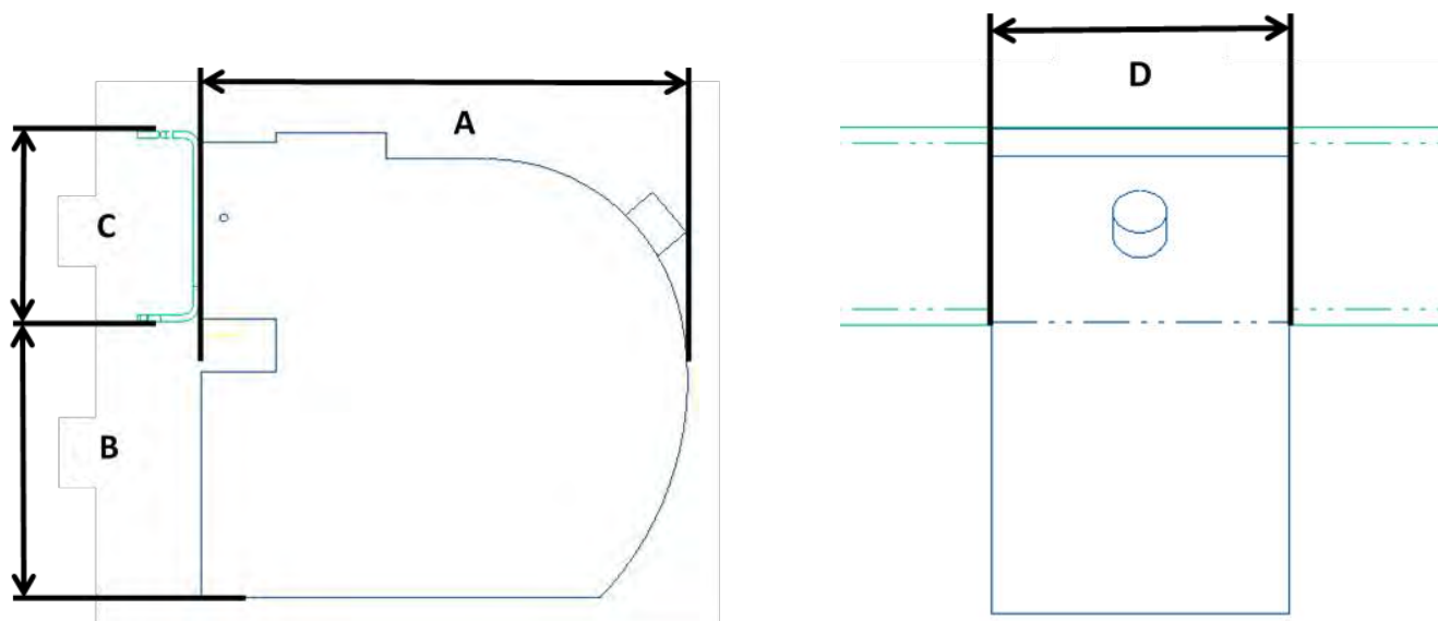
FIGURE 3-40. DEF Tank Dimensions (Medium Tank Shown)
