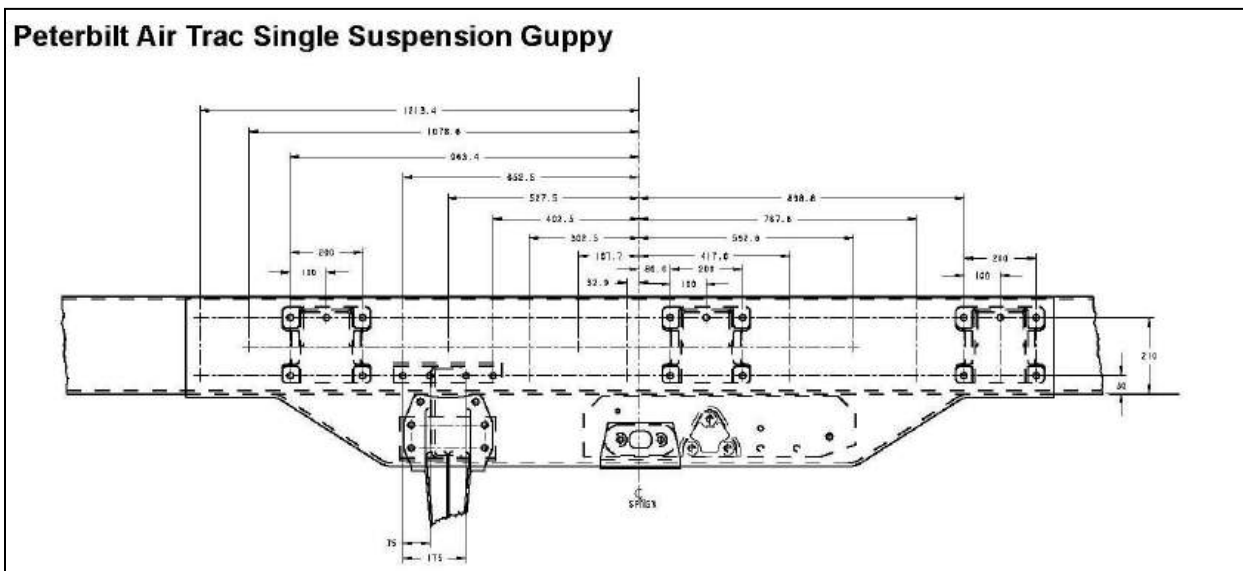
FIGURE 3-30. Peterbilt Air Trac Single Suspension Guppy
