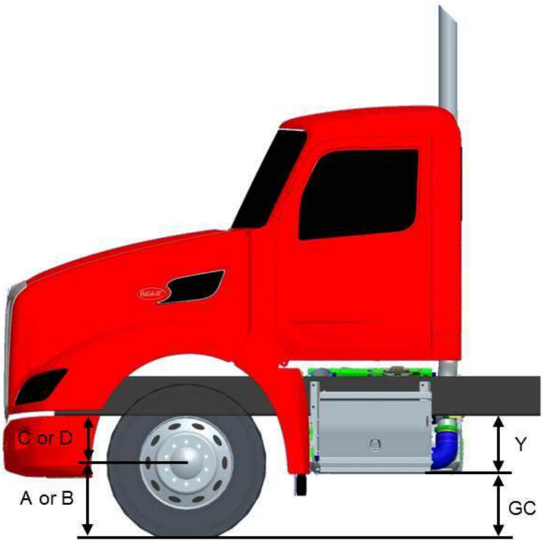
FIGURE 3-37. Ground Clearance Calculations
