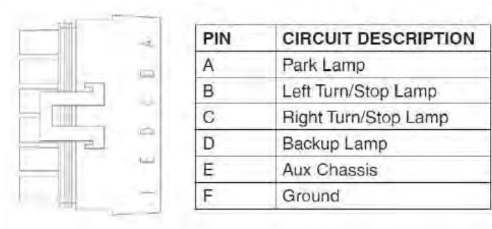
Mating Connector: Packard PN 12020786
