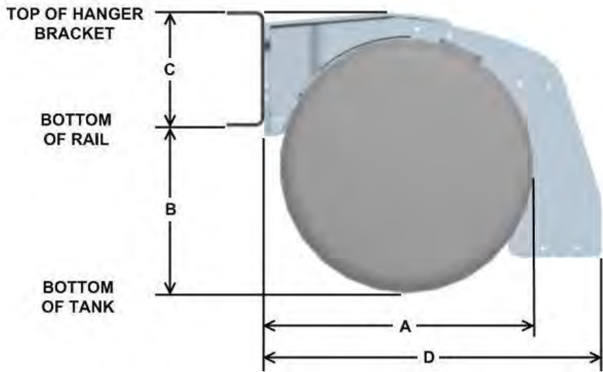
FIGURE 3-39. Fuel Tanks
