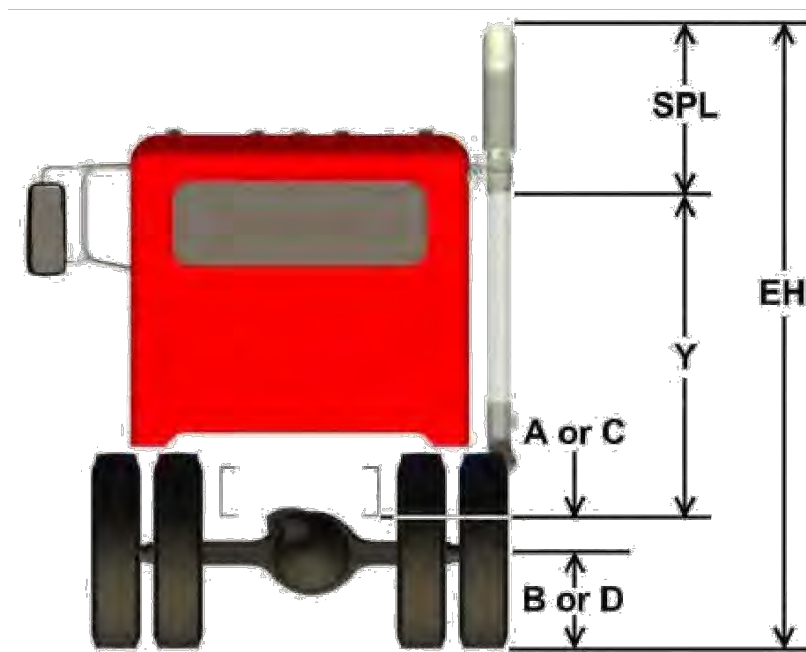
FIGURE 3-36. Exhaust Height Calculations
