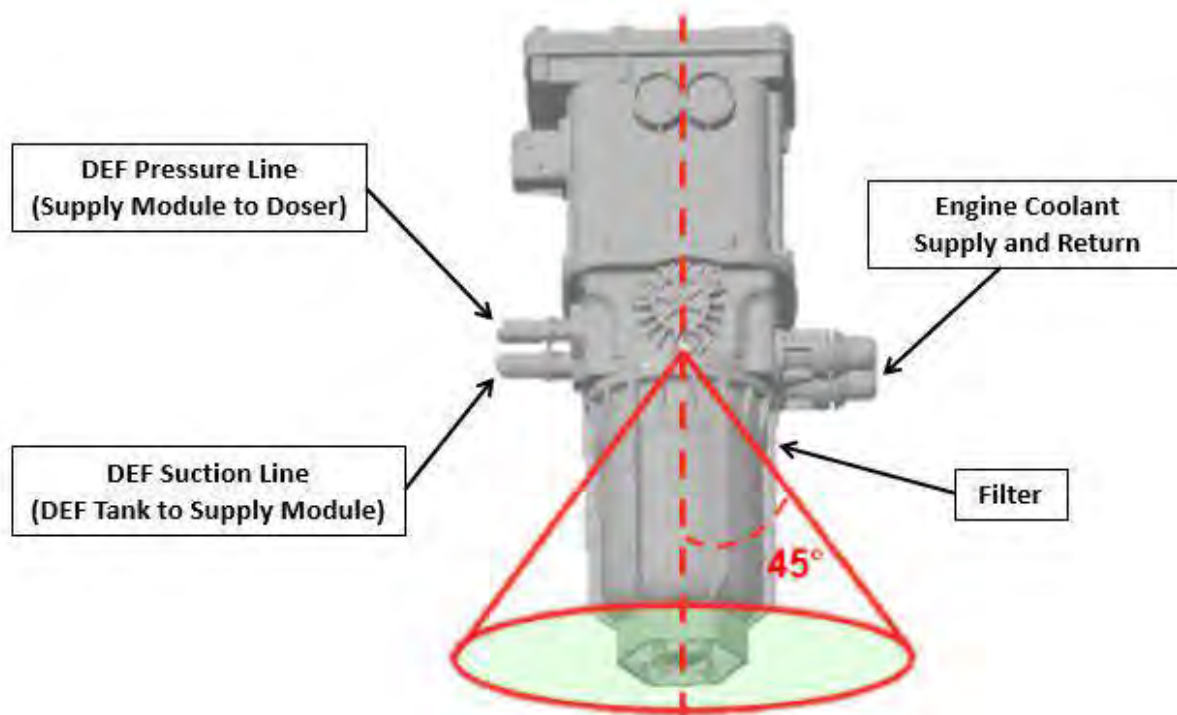
FIGURE 9-4. Supply Module Mounting Angle Limits
