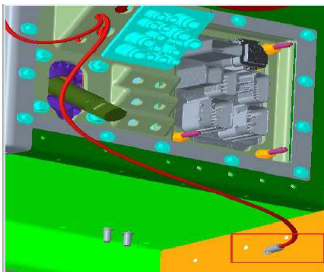
Grounding Point – Below Cab floor LH hand Cab SIL
