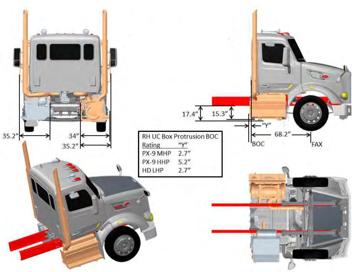
FIGURE 3-80. Exhaust Dual SOC DPF/SCR RH Under Cab
