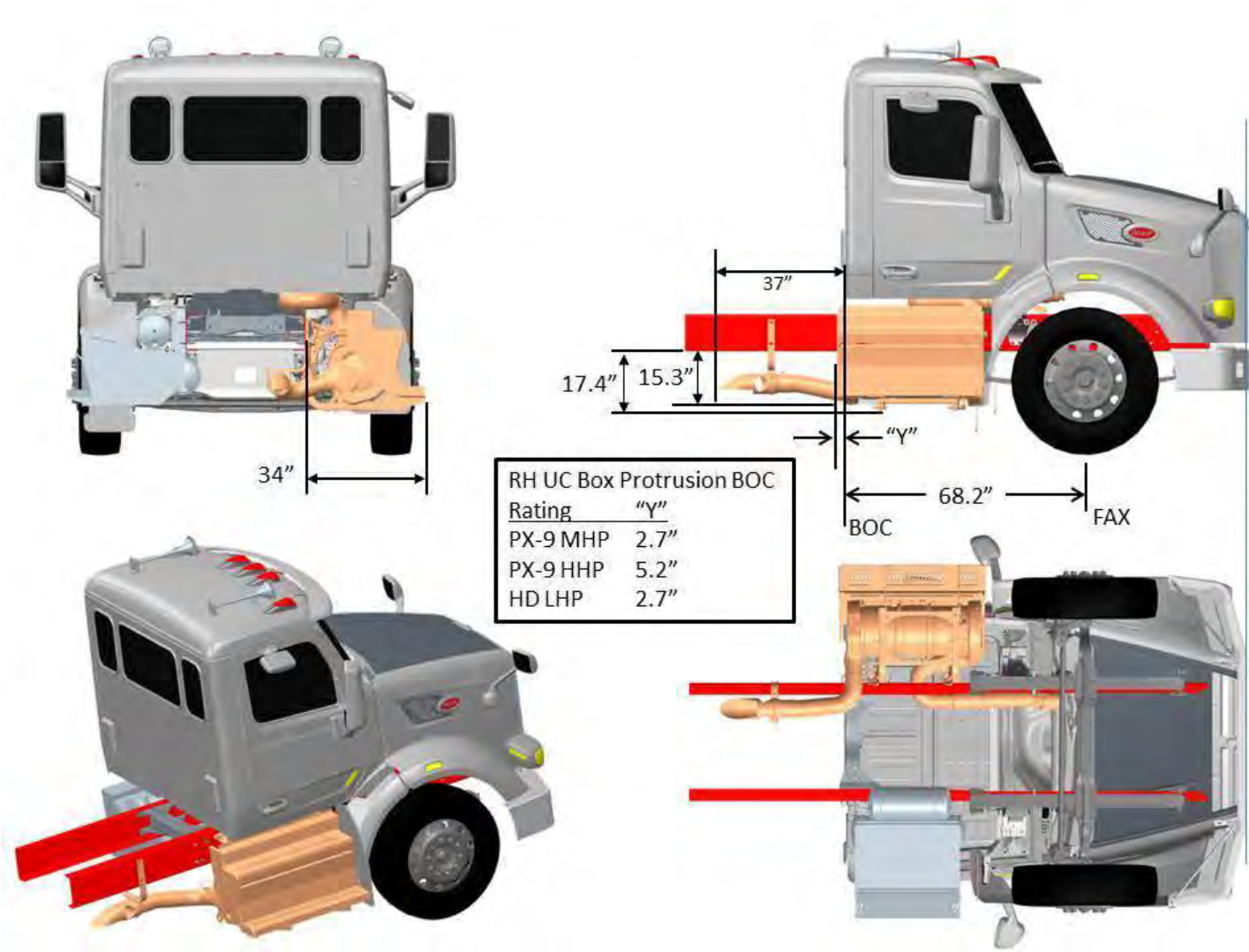
FIGURE 3-78. Exhaust Single RH Horizontal DPF/SCR RH Under Cab
