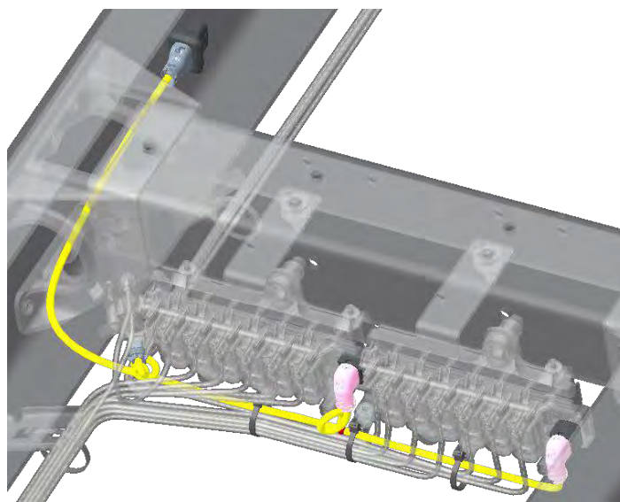
Mux Solenoid Bank
