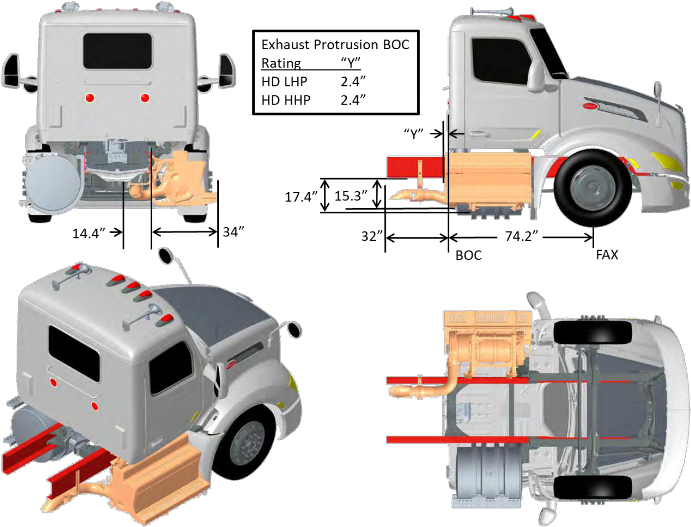
FIGURE 3-103. Exhaust Single RH Horizontal DPF/SCR RH Under Cab
